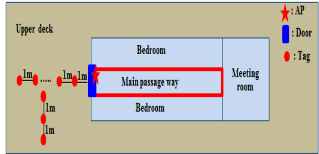
Figure 13: Test on Transmittance in upper deck and door of main passage way
