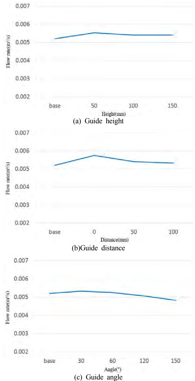
Figure 6: Induced hydrogen flow rate in the case of upward flow
