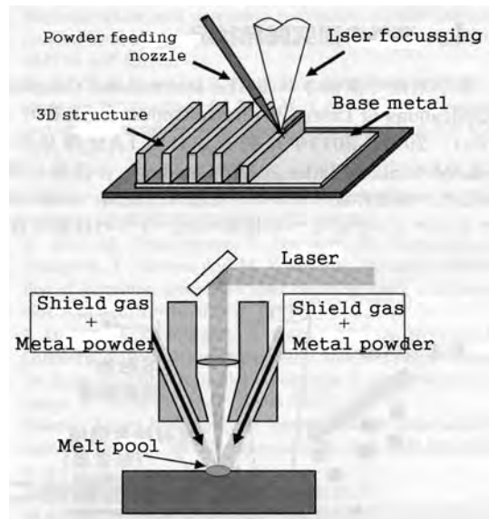
Figure 12: Schematic of LMD(Laser Metal Deposition) [13]
