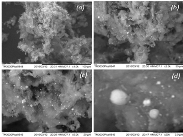
Figure 1: Typical SEM images of NiNPs/Carbon prepared by solution plasma in waste vegetable oil at various magnifications: (a) ×1000, (b) ×2500, (c) ×5000, and (d) ×20000.
