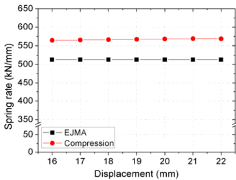
Figure 4: Comparison of spring rate by calculated EJMA and the result of FEM
