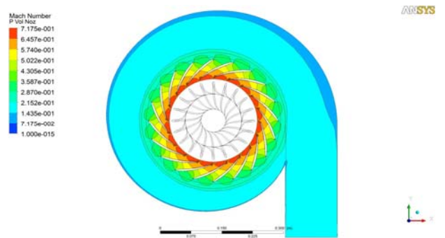
Figure 8: Mach No. distribution of the volute and nozzle
