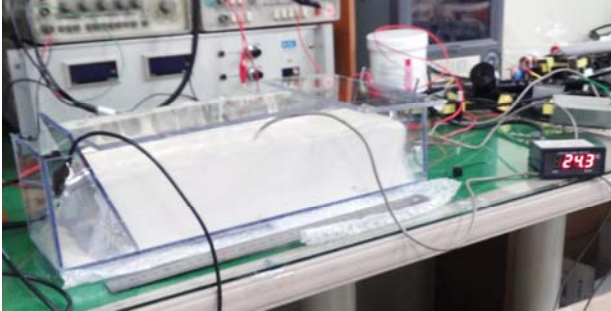
Figure 7: Exothermic properties exoeriment according to Dielectric compositions
