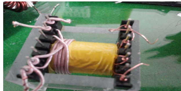
Figure 4: Self-resonant winding method
