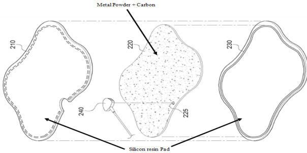
Figure 15: Structure of insulated electrode
