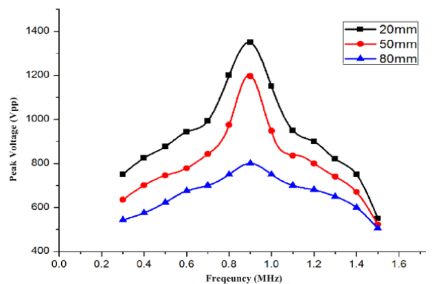
Figure 20: Voltage curve according to frequency increasing (Vpp)
