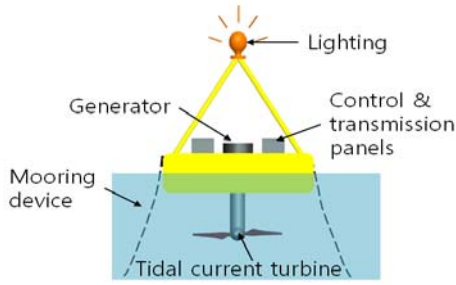
Figure 1: Schematic view of proposed floating type tidal current turbine
