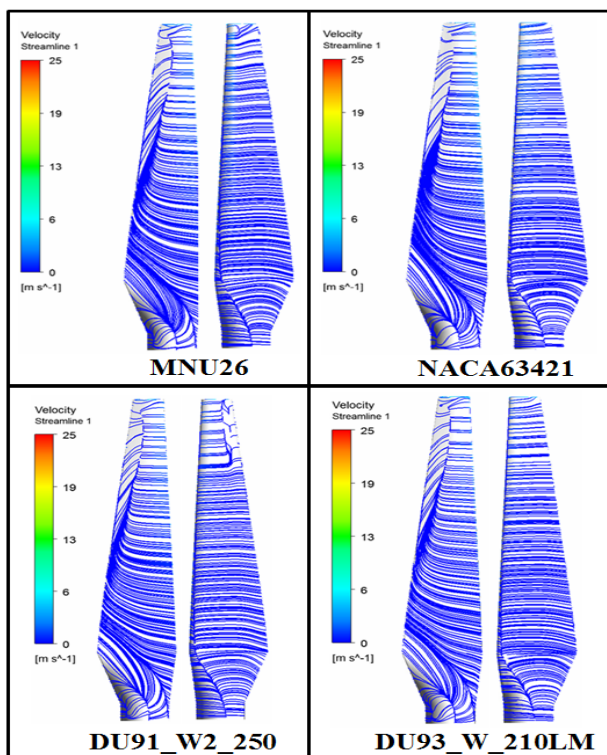
Figure 11: Streamlines on blade surface at TSR5
