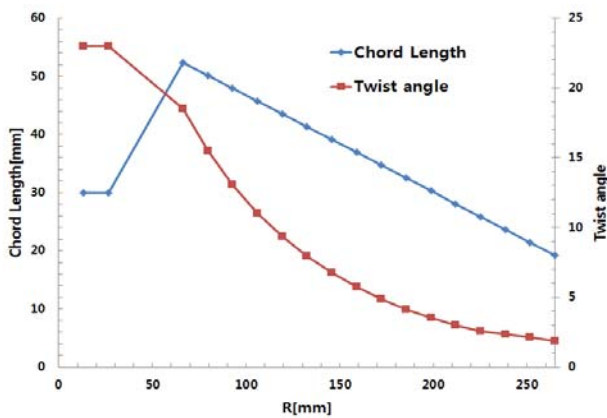
Figure 5: Twist angle, radial length and chord length of 50W class rotor blade model designed
