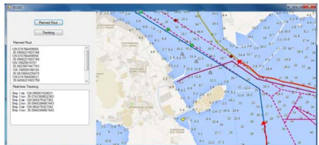
Figure 7: Creation of the ECDIS 2D visualization module
