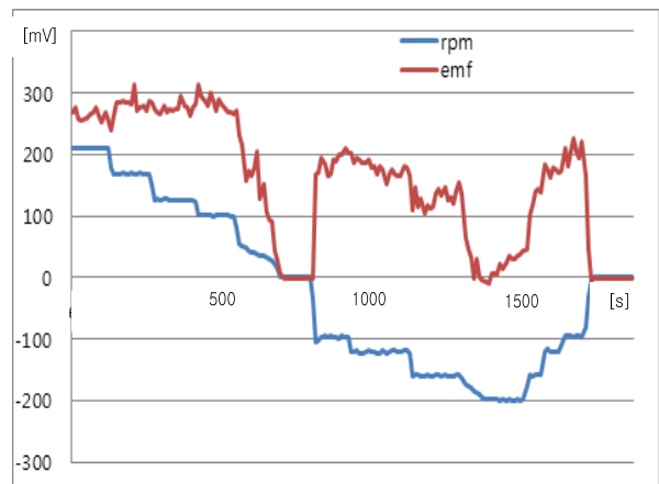
Figure 7: Characteristics of shaft EMF at forward & reverse revolution
