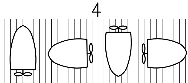
Figure 4: An effect on the EMF by Ship's heading & earth magnetic field
