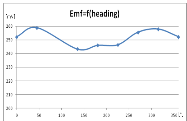
Figure 3: The amplitude of the EMF by Ship's heading
