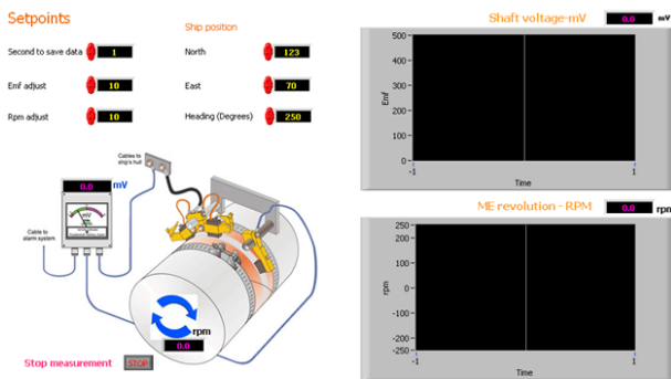
Figure 1: A schematic of the EMF measurement apparatus of ship
