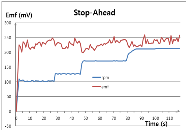
Figure 5: Characteristic of shaft EMF according to the revolution
