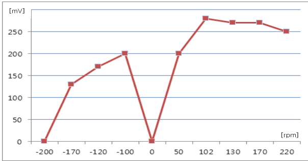
Figure 8: Characteristics of shaft EMF according to M/E RPM
