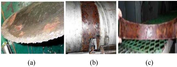
Figure 9: Photos of the damage caused by shaft EMF [4]
