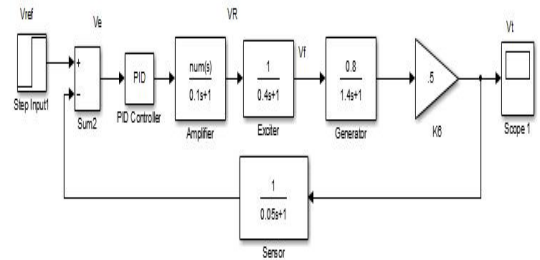
Figure 3: AVR system with PID
