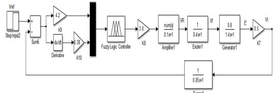
Figure 5: AVR system with FLC
