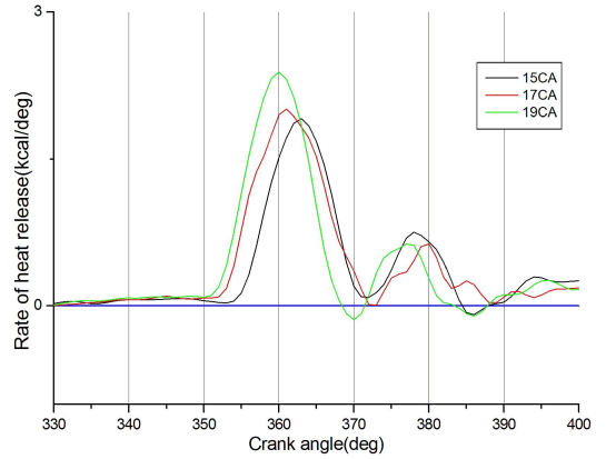
Figure 6: Rate of heat release according to adjustments fuel injection timing with the 50% load.
