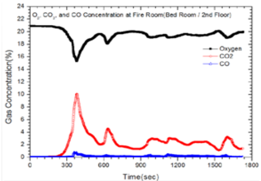
Figure 9: Gas concentration distribution in the bedroom through the fire reproduction experiment [5]
