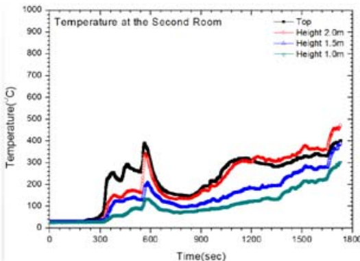
Figure 7: Temperature distribution in the Second Room through the fire reproduction experiment [5]
