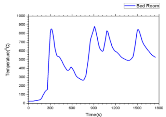
Figure 4: Temperature distribution in the bedroom by CFAST analysis [6]
