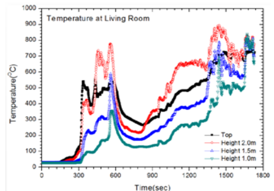
Figure 5: Temperature distribution in the Living Room through the fire reproduction experiment [5]
