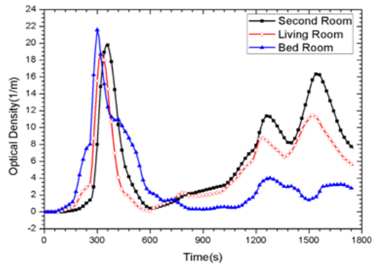
Figure 12: Optical Density in rooms
