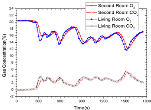
Figure 11: Gas concentration distribution in the room by CFAST analysis
