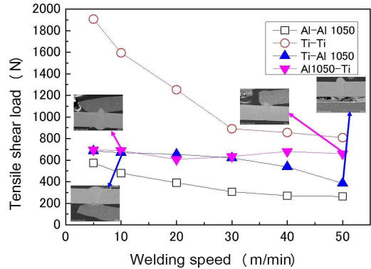
Figure 6: Results of tensile shear test for Ti and Al similar and dissimilar welds with single-mode laser.
