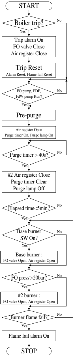
Figure 3: Flow diagram for burner control
