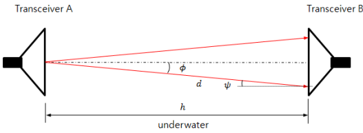
Figure 1: Basic schematic of the underwater communication channel.
