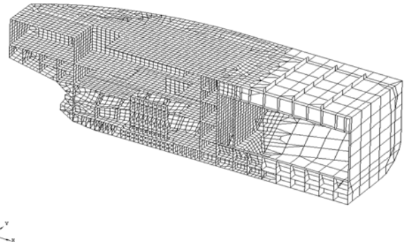
Figure 3: FE model of 50,000 DWT oil/chemical tanker
