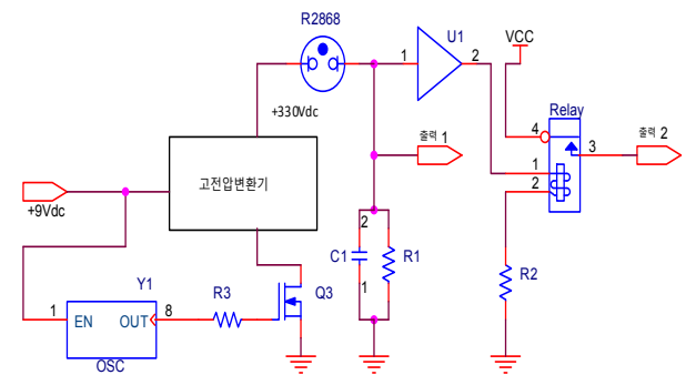
Figure 3: Driving circuit of R2868
