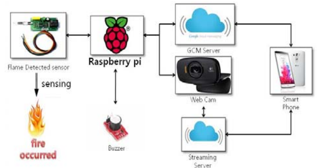
Figure 2: System configuration
