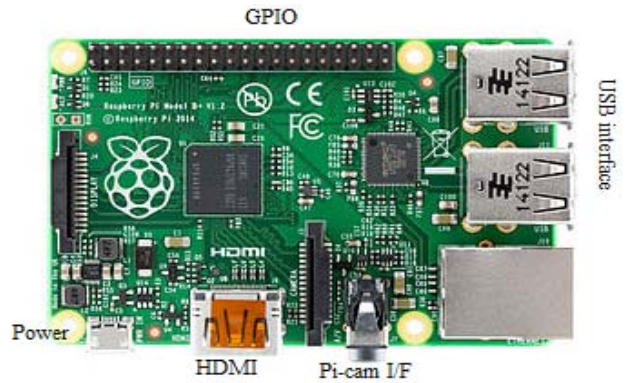
Figure 1: Raspberry Pi B+
