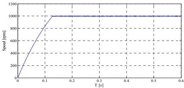
(a) 0 → 1000[rpm]
