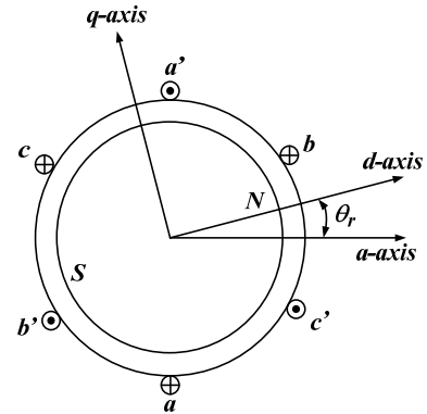
Figure 3: Model of BLDC Motor
