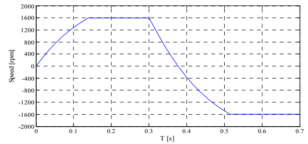
(b) 1600 → -1600[rpm]
