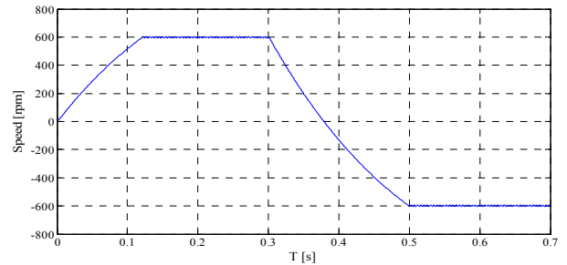
(a) 600 → -600[rpm]
