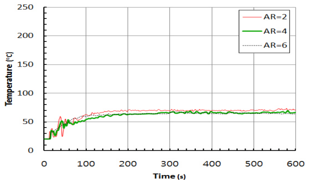
(b) 1 [MW] in enclosure L
