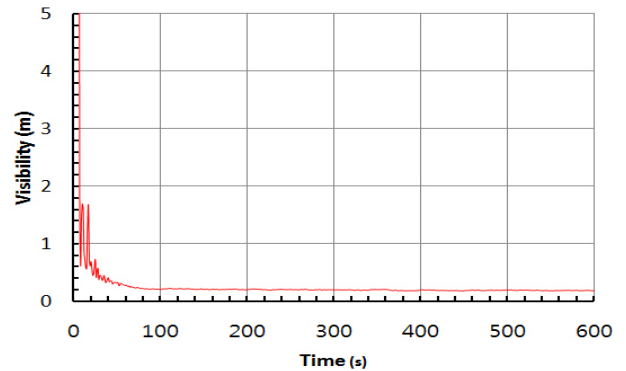
(c) visibility at point P 1
