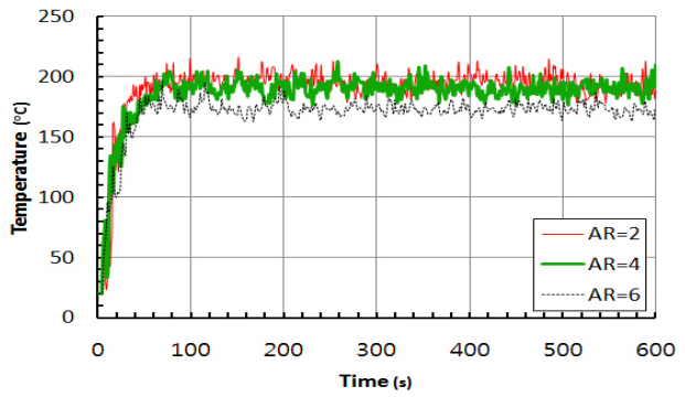
(c) 2 [MW] in enclosure S
