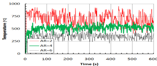
(c) 2 [MW] in enclosure S
