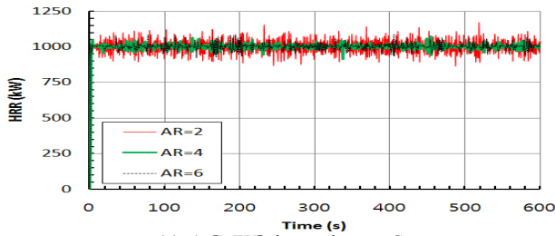
(a) 1 [MW] in enclosure S
