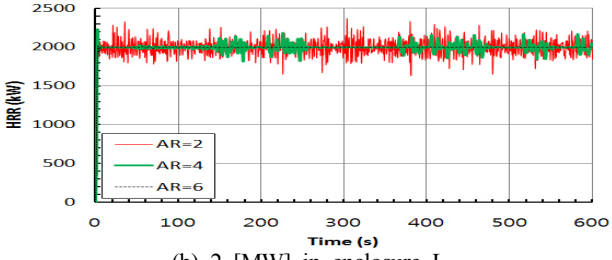
(b) 2 [MW] in enclosure L
