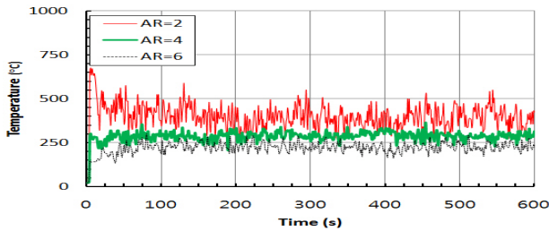
(a) 1 [MW] in enclosure S
