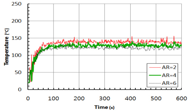
(a) 1 [MW] in enclosure S
