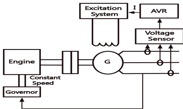
Figure 1: Configuration of Excitation System of Brushless Synchronous Generator on board ship[12]
