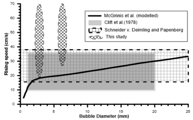
Figure 4. Compiled data of rising speed against bubbles size (modified from Greinert et al. 2006 [6])
