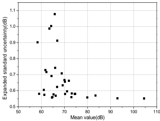
Figure 5: Uncertainty distributions of “C” class ship
