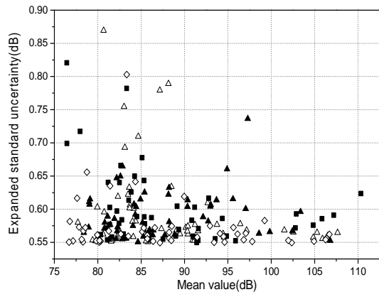
Figure 3: Uncertainty distributions of “A” class ship
