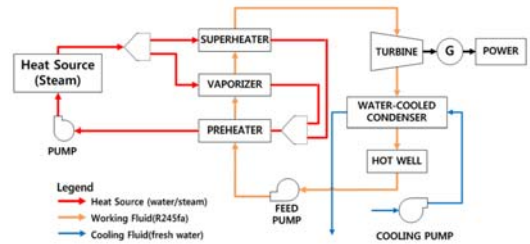
Figure 5: Design of a Superheater Parallel Connection
