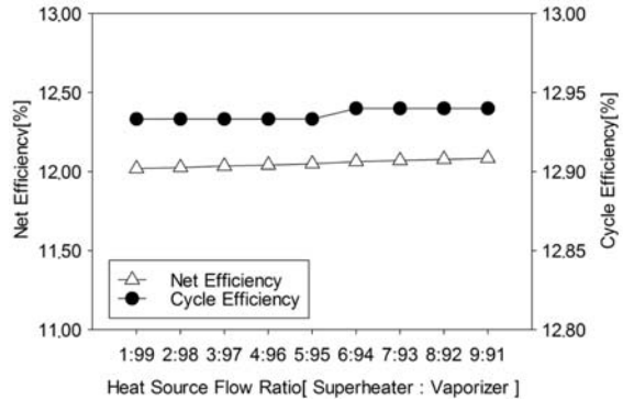
Figure 7: Diagram of Vapor Fraction
