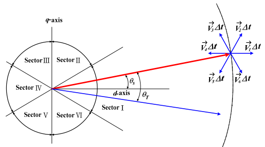
Figure 2: Principle of direct torque control
