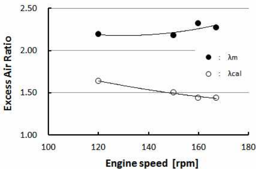
Figure 8: Comparison of excess air ratio \lambda_m and \lambda_{cal} for fitting to measurement results.
